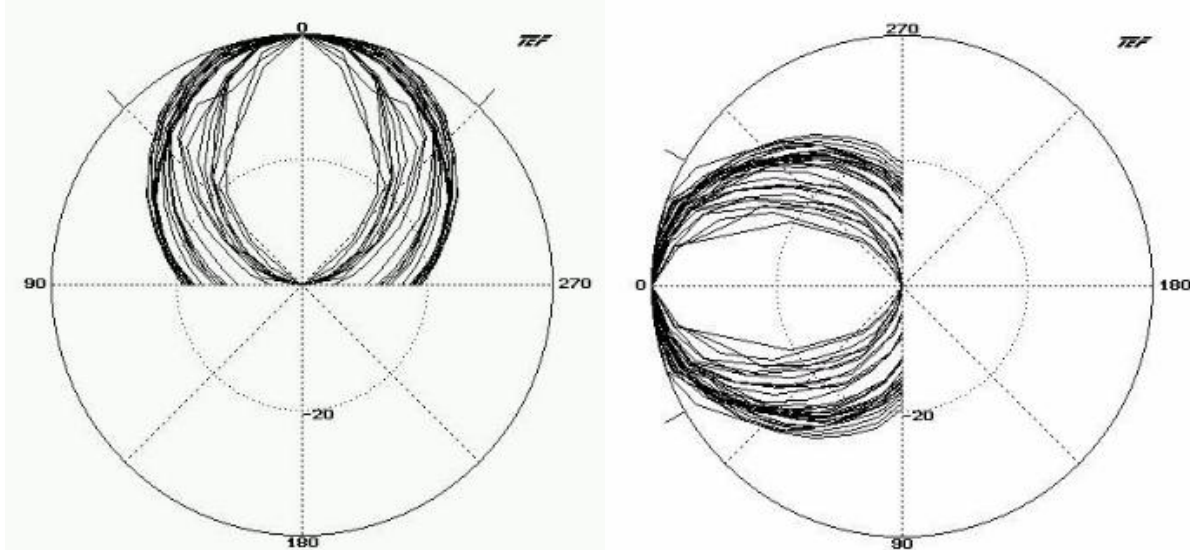
Horizontal & Vertical Polar Response, 630Hz - 16kHz 1/6 octave center frequencies
