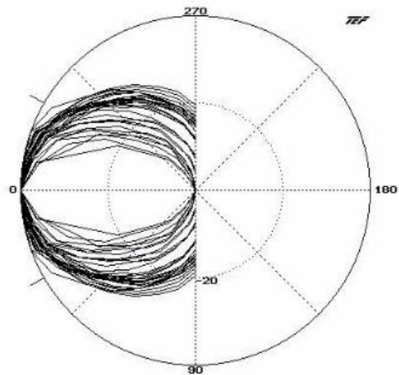
Horizontal & Vertical Polar Response, 630Hz - 16kHz 1/6 octave center frequencies
