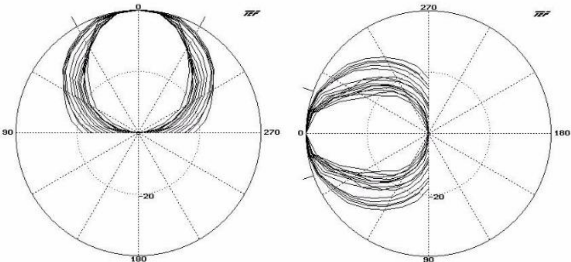
Horizontal & Vertical Polar Response, 630Hz - 16kHz 1/3 octave center frequencies
