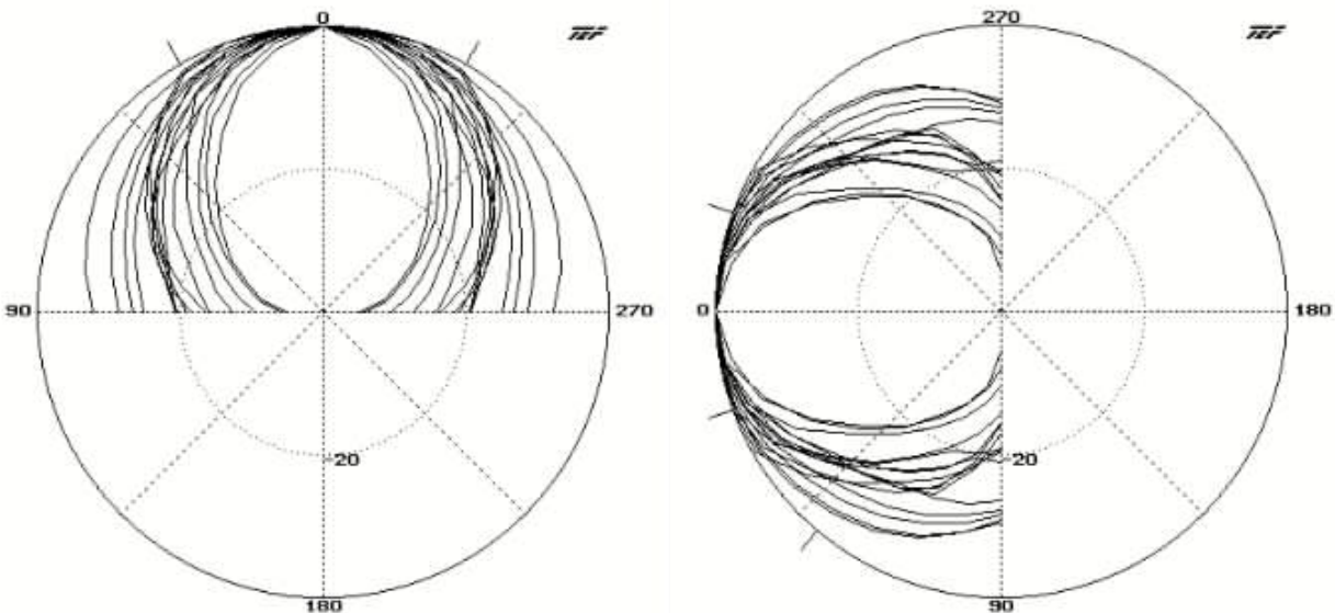
Horizontal & Vertical Polar Response, 630Hz - 16kHz 1/6 octave center frequencies
